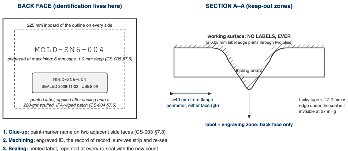
Figure 2: Figure 2. Where a mold's identity lives, and the two keep-out zones: never the working surface, never within 40 mm of the flange perimeter on either face.
